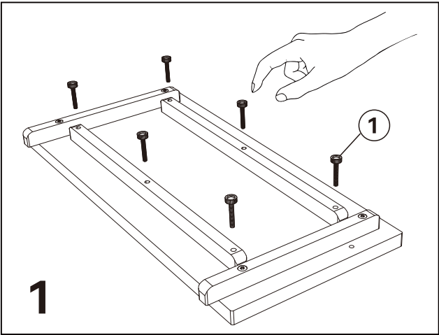
Remove battens from extension leaf
