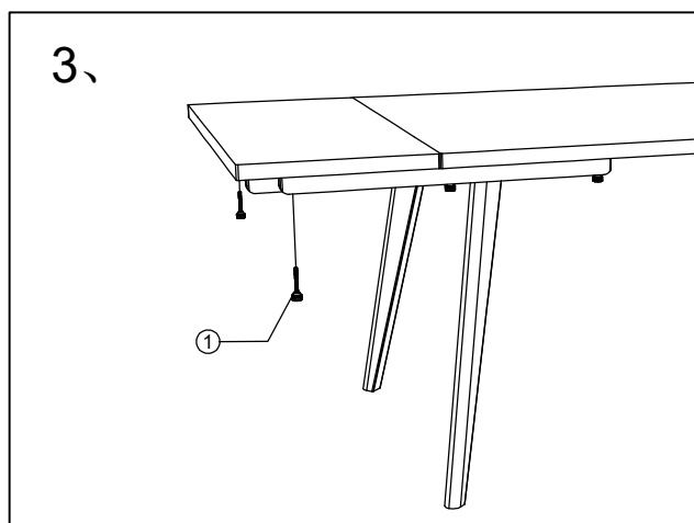
Secure extension leaf with 2 more thumbscrews
