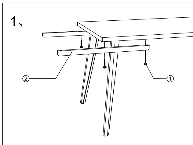
Attach battens with thumbscrews
